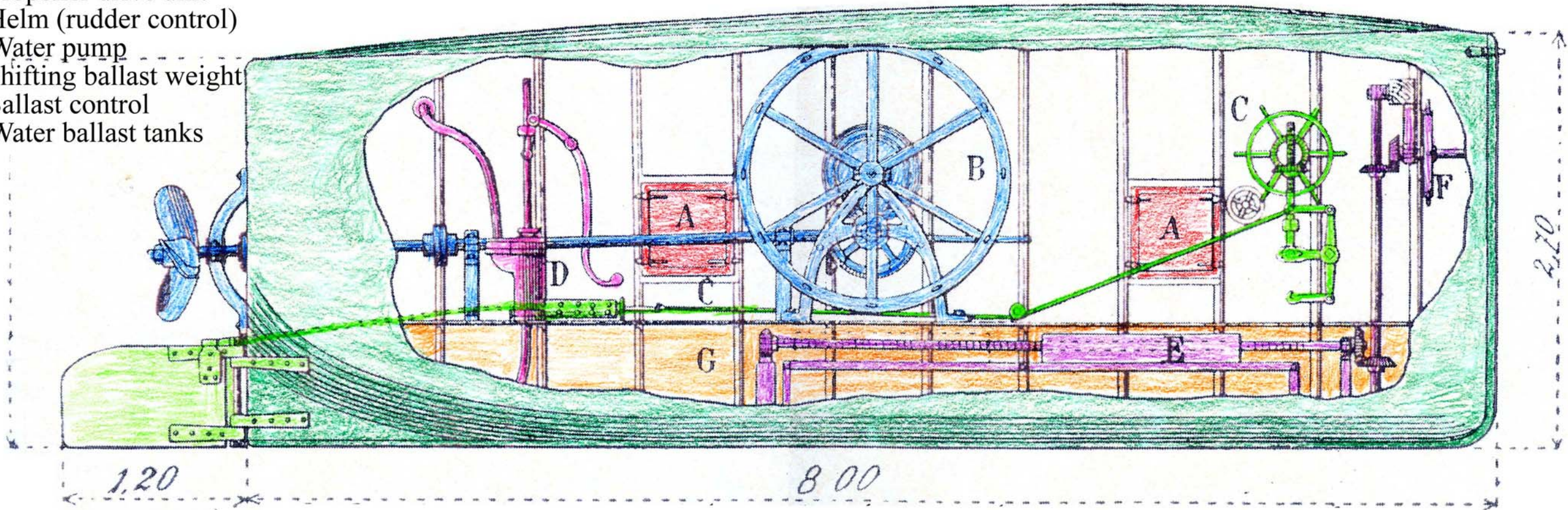
Bauer's submarine design, said to have been built by the special order of Duke Constantine of Russia, performed quite well. It made 100 dives near St. Petersburg and stayed submerged for 6-8 hours.
